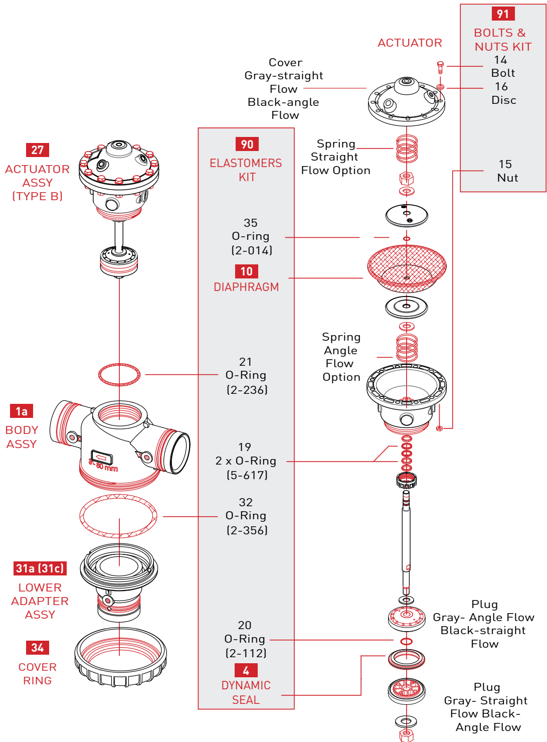
31a - LOWER ADAPTER ASSY WITH 2" THREAD (STRAIGHT FLOW) 31c - LOWER ADAPTER ASSY - GROOVED (ANGLE FLOW)
